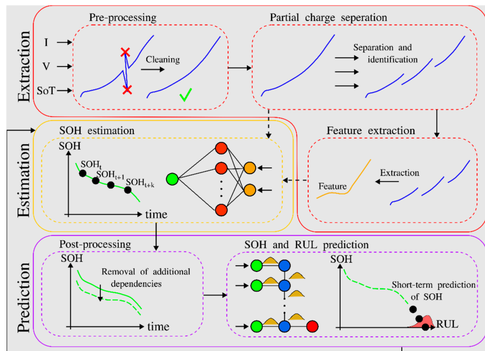
Figure 8. A flowchart of the Smart Battery SOH and RUL prediction framework. In order to stabilize the predictions of the SOH, the time dependence of the system is moved from the SOH to the features. To predict the SOH, the features are predicted forward in time, and a SOH estimation model is then used to predict the SOH.
