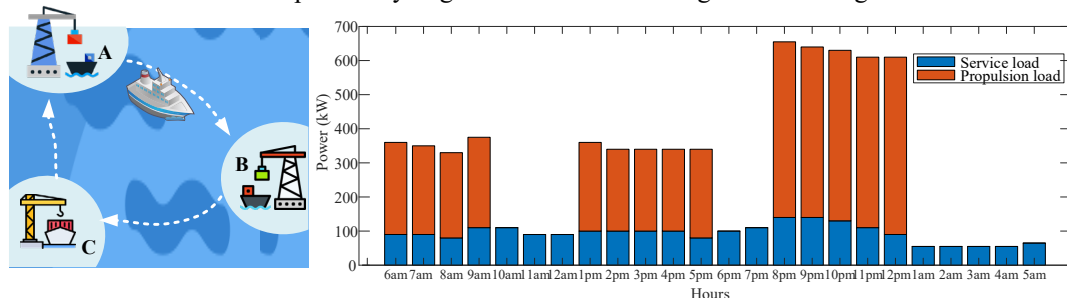
Fig. 1. (a) vessel routine example; (b) onboard loads for one day.
