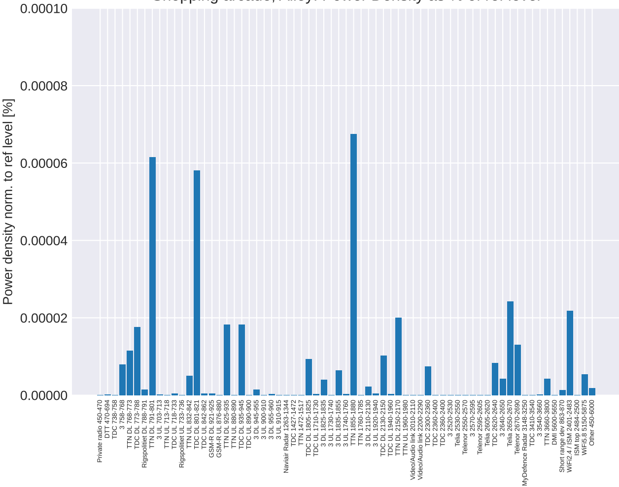
Shopping arcade, Alley: Power Density as % of ref level
