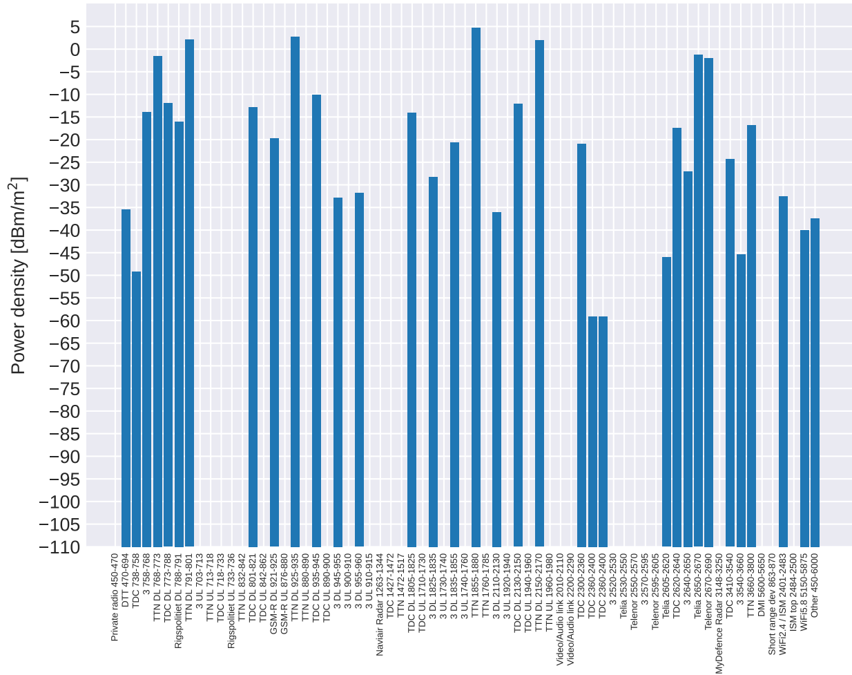
Salling Rooftop: Power density
