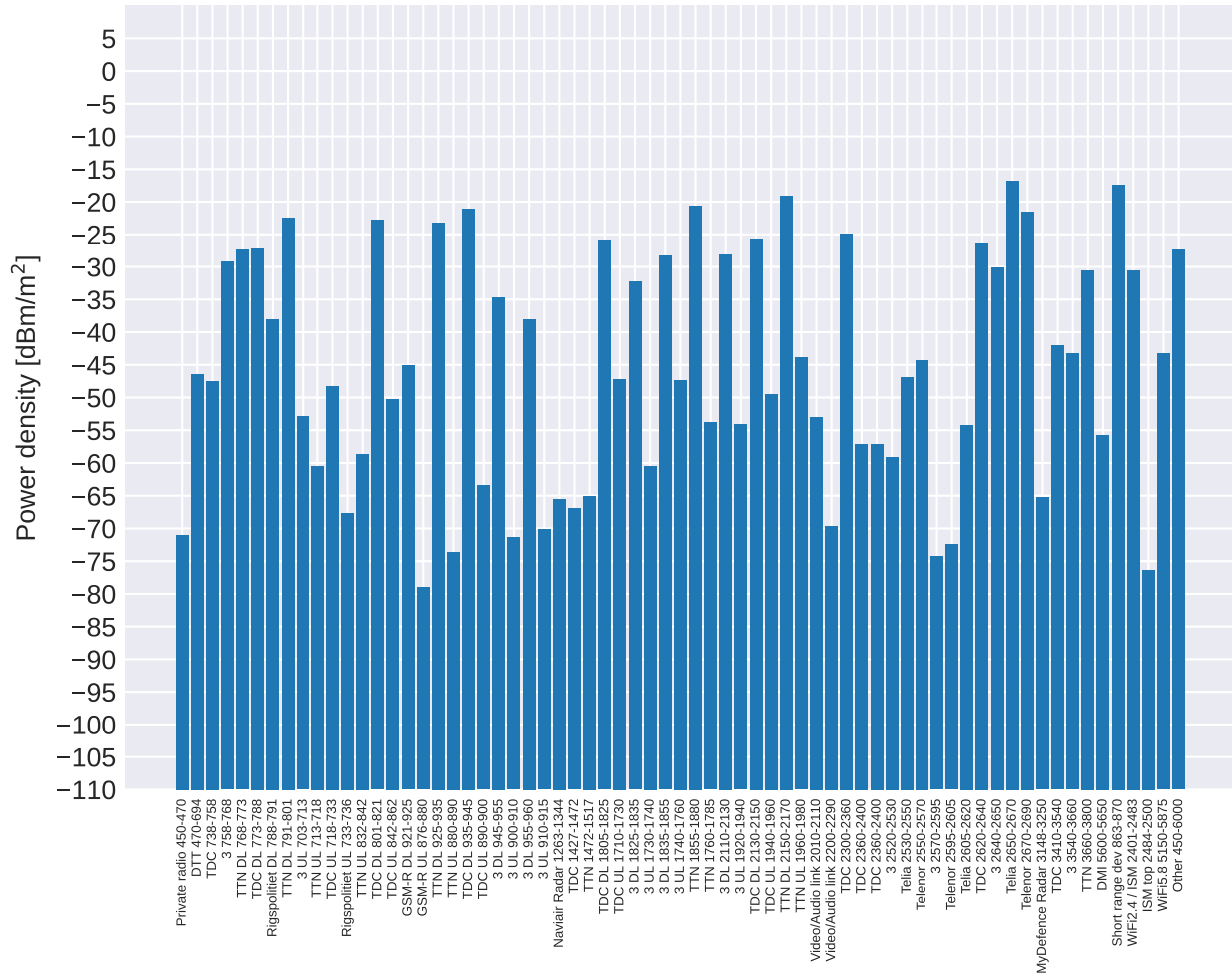
Shopping arcade, Center: Power density
