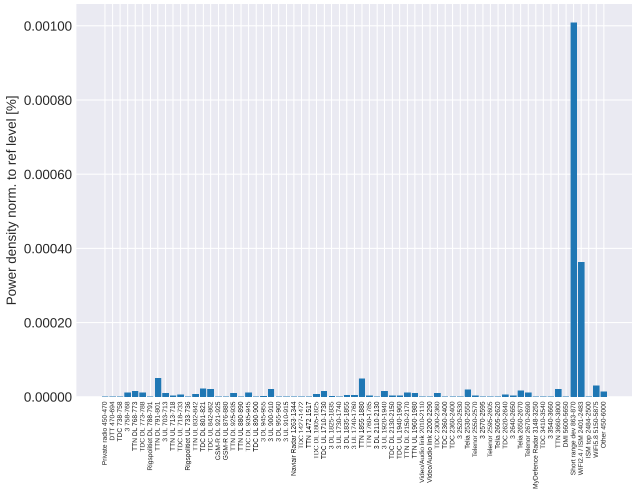
Shopping arcade, Bilka: Power Density as % of ref level
