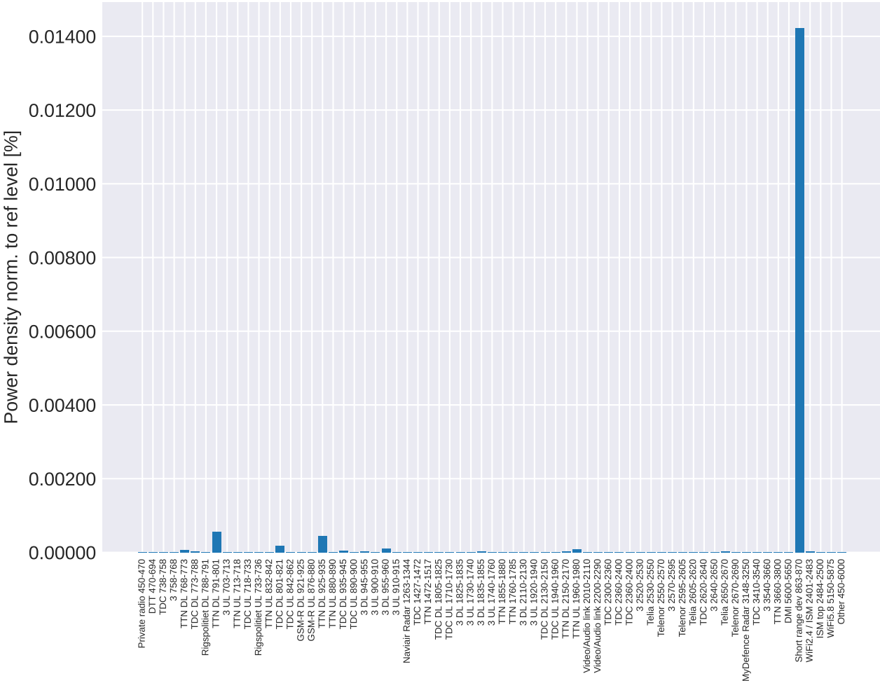
Airport Entry: Power Density as % of ref level
