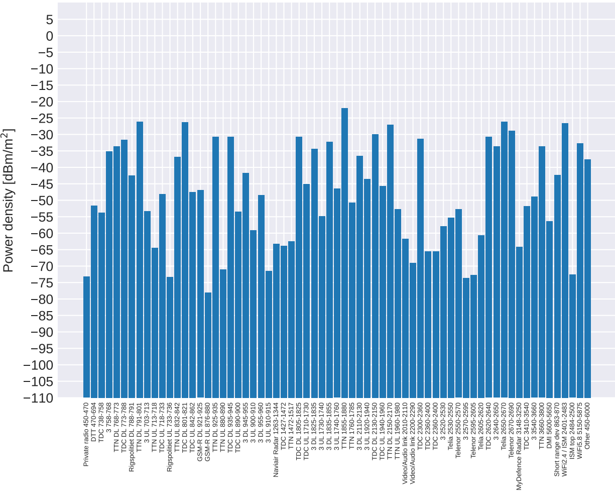
Shopping arcade, Alley: Power density
