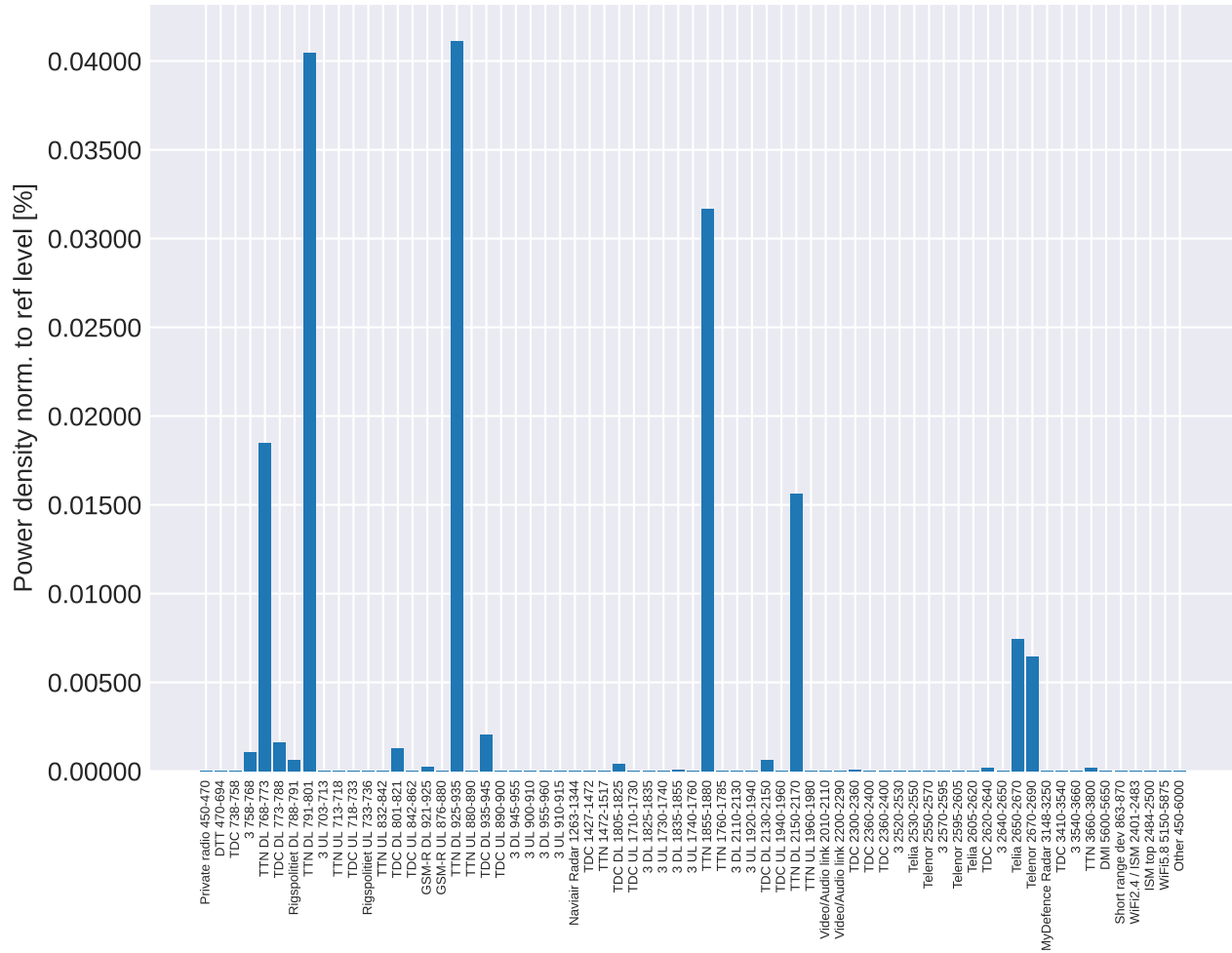
Salling Rooftop: Power Density as % of ref level
