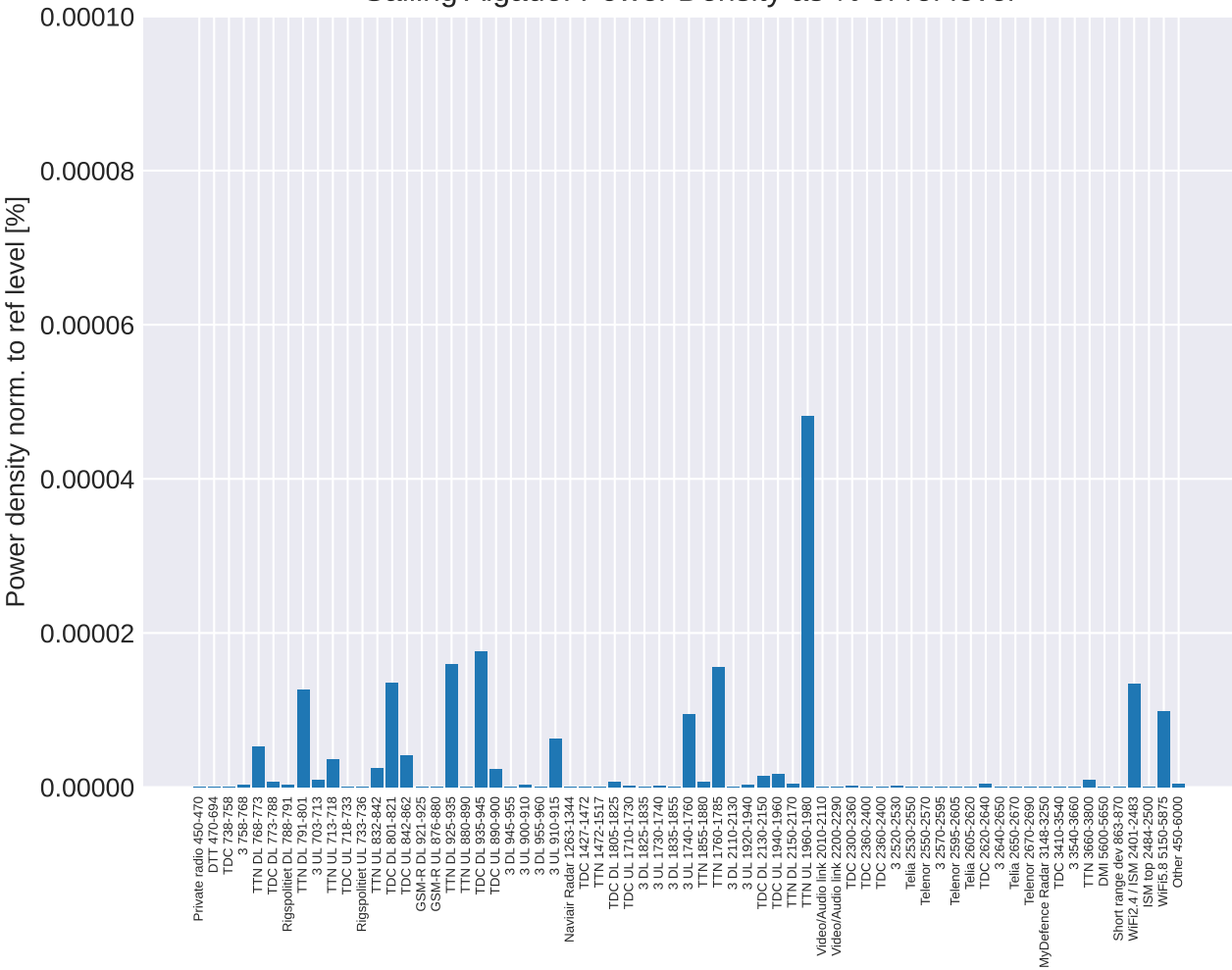
Salling Algade: Power Density as % of ref level
