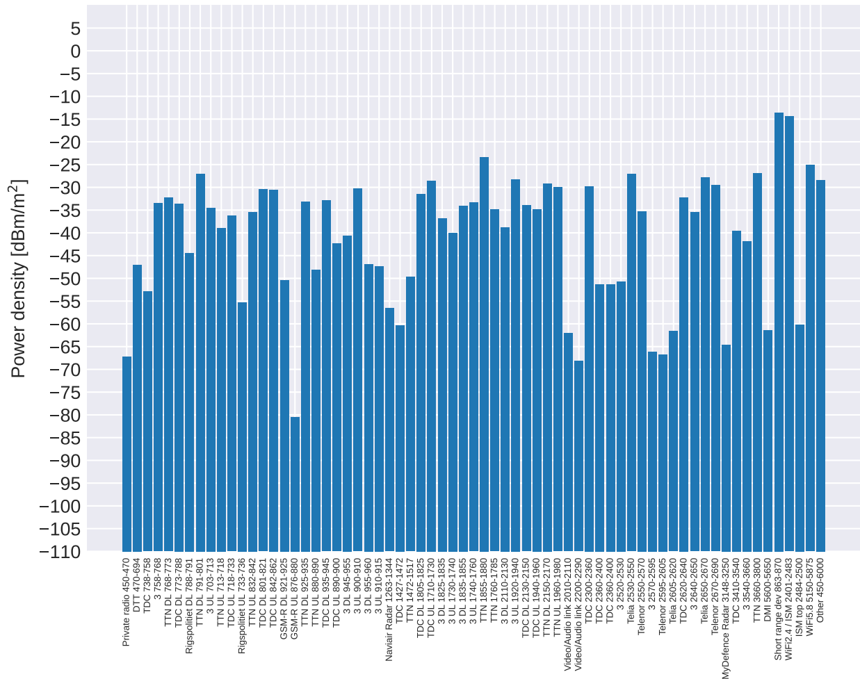
Shopping arcade, Bilka: Power density
