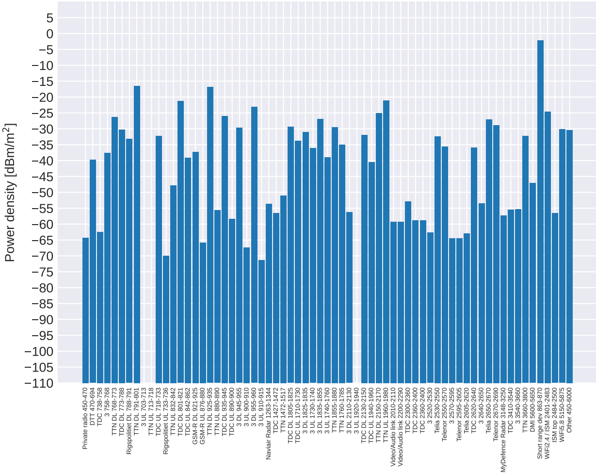
Airport Entry: Power density
