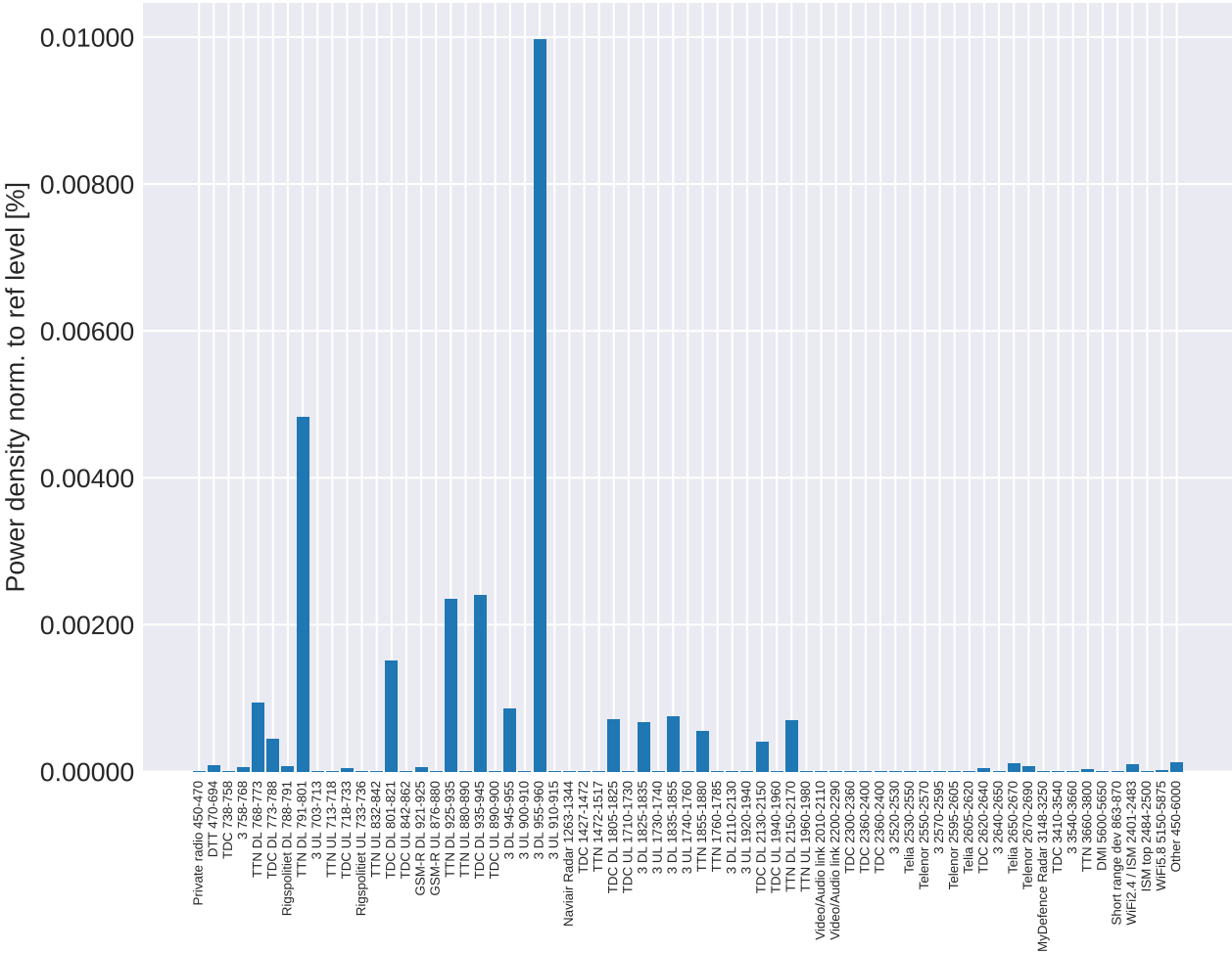
Airport Gate: Power Density as % of ref level
