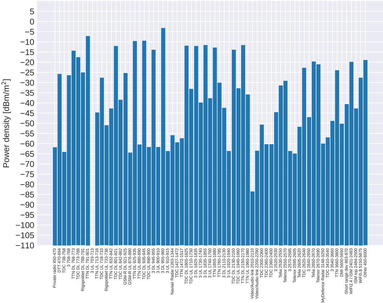
Airport Gate: Power density
