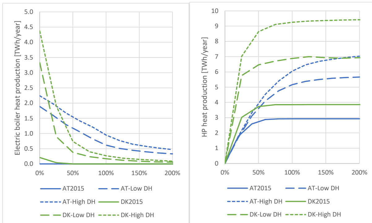
Figure 7: DH production of the electric boilers and HPs in the scenarios. The x-axis shows the installed electric boiler capacity. For the AT scenarios 100% on X-axis correspond to 1.2 GWe HP capacity, and for DK scenarios 100% correspond to 2.3 GWe HP capacity.
