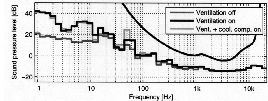
Figure 5: Third-octave analysis of the background noise measured at the listening position in the low-frequency test facility compared to the diffuse-field pure-tone hearing threshold [45]: Ventilation off, ventilation on, and ventilation and cooling compressor on. Values above approx. 2000 Hz reflect the noise-floor of the measurement microphone and preamplifier.
