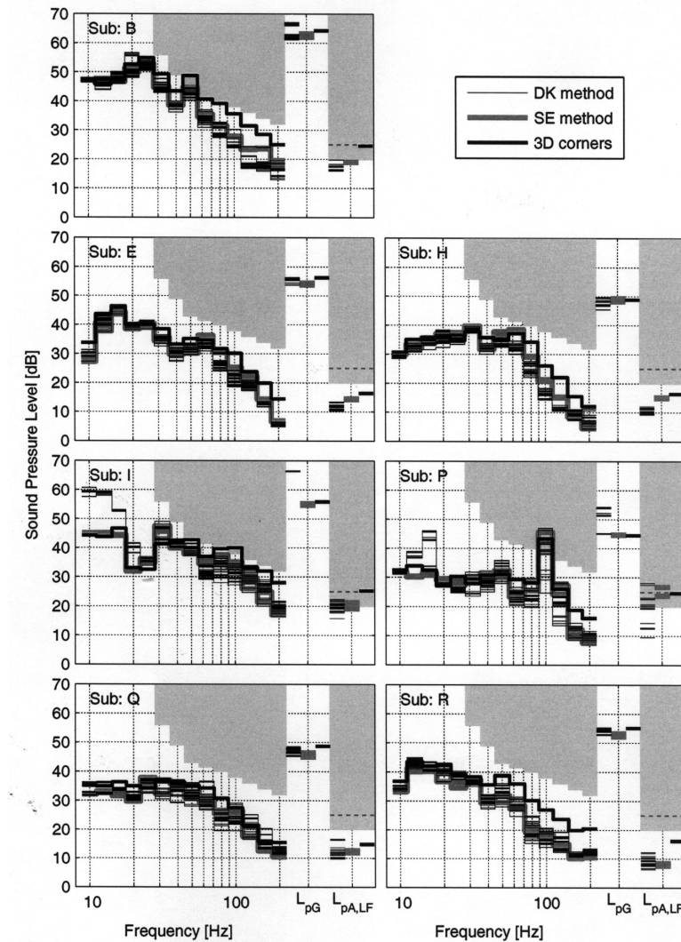
Figure 13: Comparison of all possible outcomes of the measurement methods compared to the Danish and Swedish limits. The grey areas represent the limits in Denmark (for L_{pA,LF} ) and Sweden (for third-octave levels). The Danish L_{pG} limit of 85 dB is above the scale and not shown. For the L_{pG} and L_{pA,LF} the lines are plotted in the order: DK method, SE method, and 3D corners.
