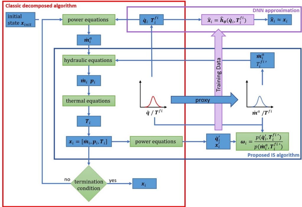
Figure 1: A DNN can be used to approximate a state estimator (purple box). We propose a new IS algorithm (blue box) to generate training samples for such a DNN. Opposite to the classic decomposed method for state estimations (red box), the IS algorithm solves the hydraulic, thermal and power equations only once per training sample.
