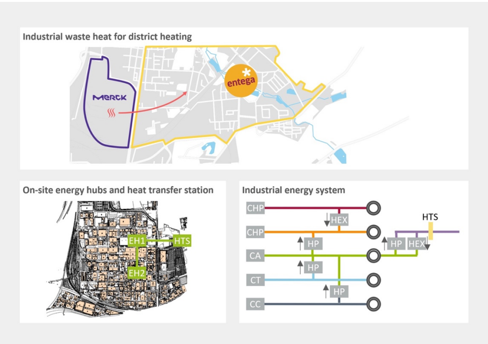
Figure caption: Interacting energy-optimized industrial district (EH: Energy hub, HTS: Heat transfer station, CHP: Combined heat and power, CA: Compressors for pressurized air, CT: Cooling tower, CC: Compression chiller, HEX: Heat exchanger, HP: Heat pump, colored lines: heating and cooling networks on different temperature levels)
