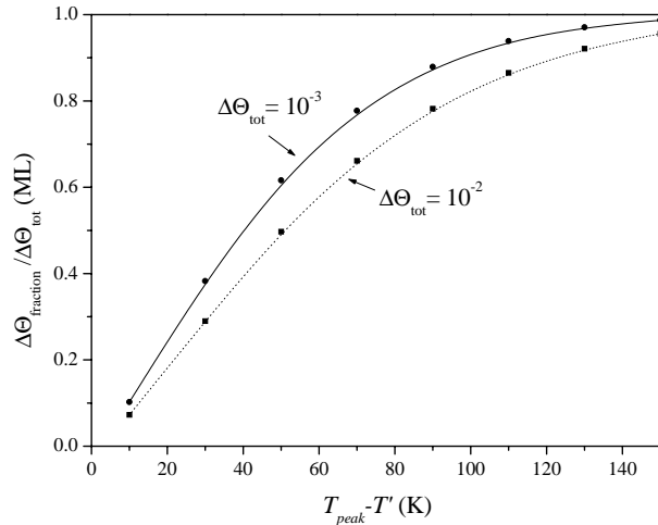
Figure 27. “The distribution in temperature“, i.e. the fraction desorbed as a function of temperature interval from the peak temperature. The peak temperatures and intensities were 643 and 733 K, and 7.2 and 8.7 MW/cm 2 for \Delta\Theta_{tot}=1\cdot 10^{-3} and 1\cdot 10^{-2} , respectively.
