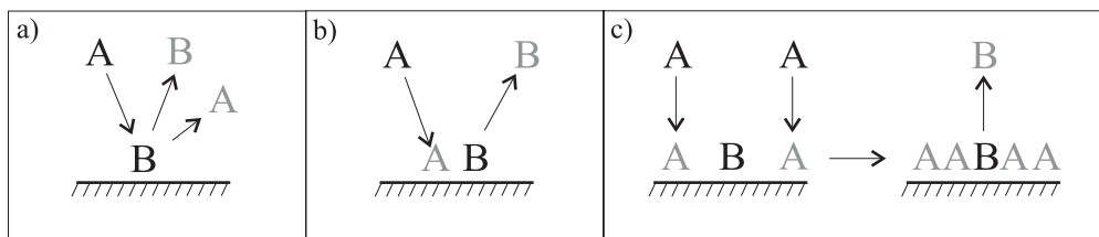
Figure 10. Three mechanisms for adsorption-induced desorption: a) Collision-induced desorption, b) Dynamic displacement, c) Thermodynamic displacement. A is the incident particle and B is the pre-adsorbed species. Black letters refer to before and gray letters refer to after “reaction”.
