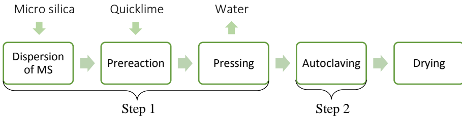
Figure 1-1 Flow diagram over the calcium silicate production process used at the Skamol A/S plant in Branden, Denmark.
