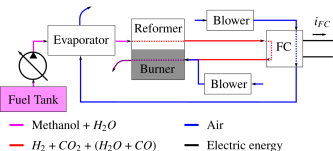
Figure 2: Diagram of the Serenus H3-350 Reformed Methanol Fuel Cell system produced by Serenegy®.
