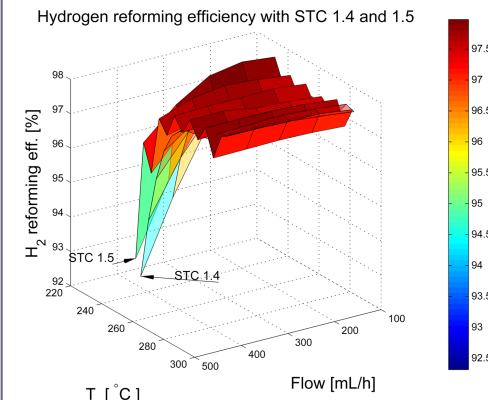
Figure 6: Surface plot of the \text{H}_2 reforming efficiency in the experiment.
