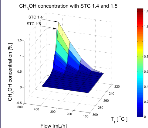
Figure 5: Surface plot of the \text{CH}_3\text{OH} concentration in the experiment.
