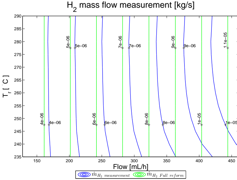
Fig. 3.28: Countour plot of the H_2 flow measured in the identification experiment.
