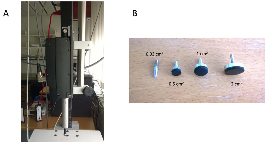
Figure 4. (A) The computer-controlled pressure algometer. (B) The four different probes used in the experiments.
