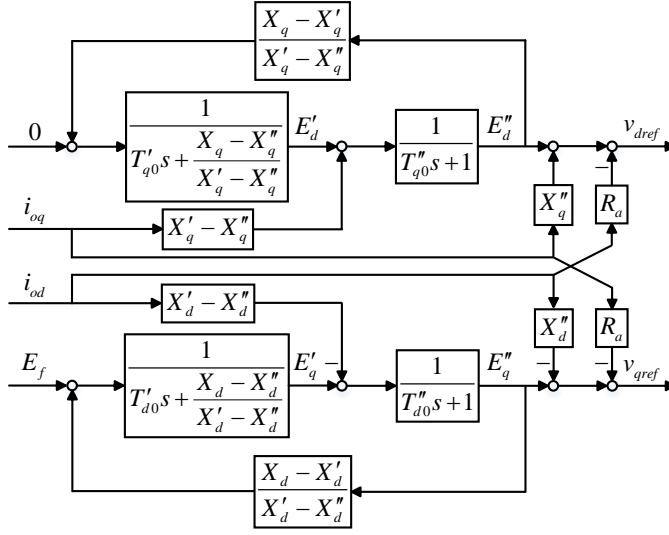
Fig. 2.2: Block diagram of virtual winding of 6th-order model based SSSG in Fig. 1.3(b). X_d and X_q are the d - and q -axis virtual synchronous reactances. Source: [C2].
