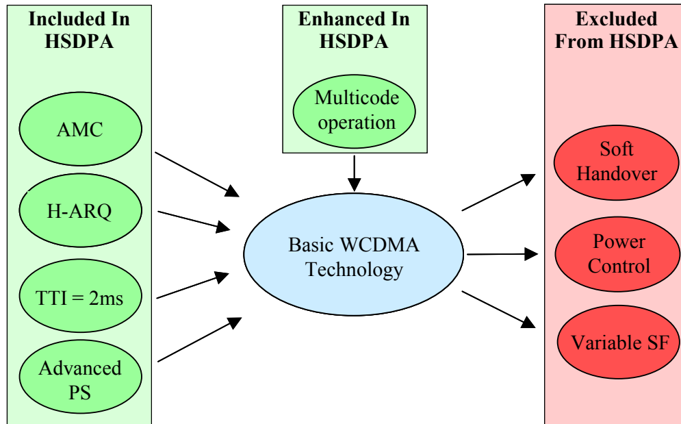
Figure 4.1: Fundamental Features To Be Included And Excluded in the HS-DSCH of HSDPA.
