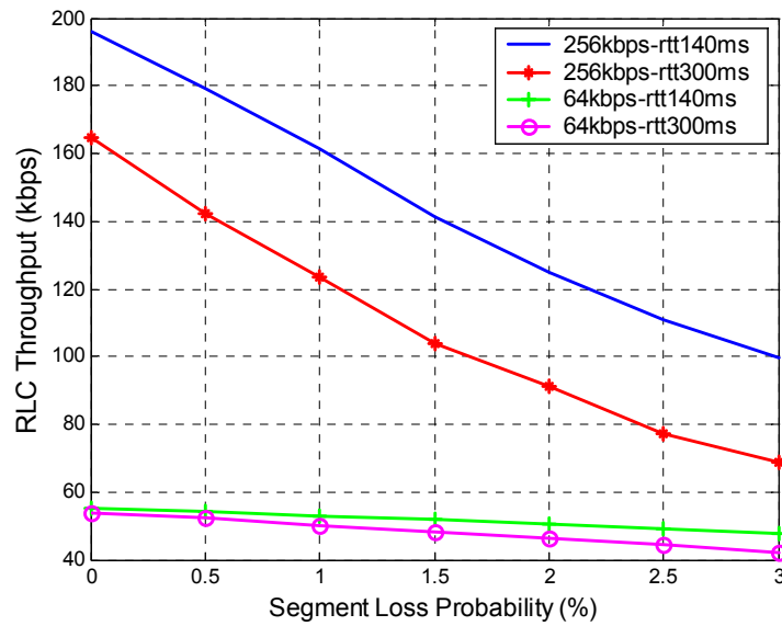
Figure 3.6: RLC Throughput as Function of the Random Segment Loss Probability for Various BDPs.
