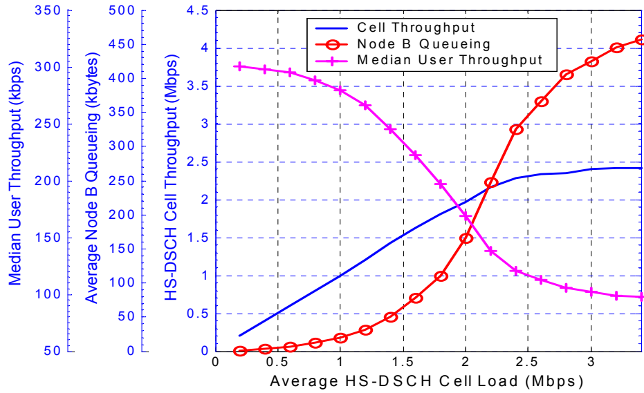
Figure 6.3: Median User Throughput, Average Node B Queueing and HS-DSCH Cell Capacity as a function of the Offered HS-DSCH Cell Load for Proportional Fair Scheduler in Pedestrian A, 3km/h. HSDPA Power \approx 50% of Total Node B Power & 7 Multi-codes.
