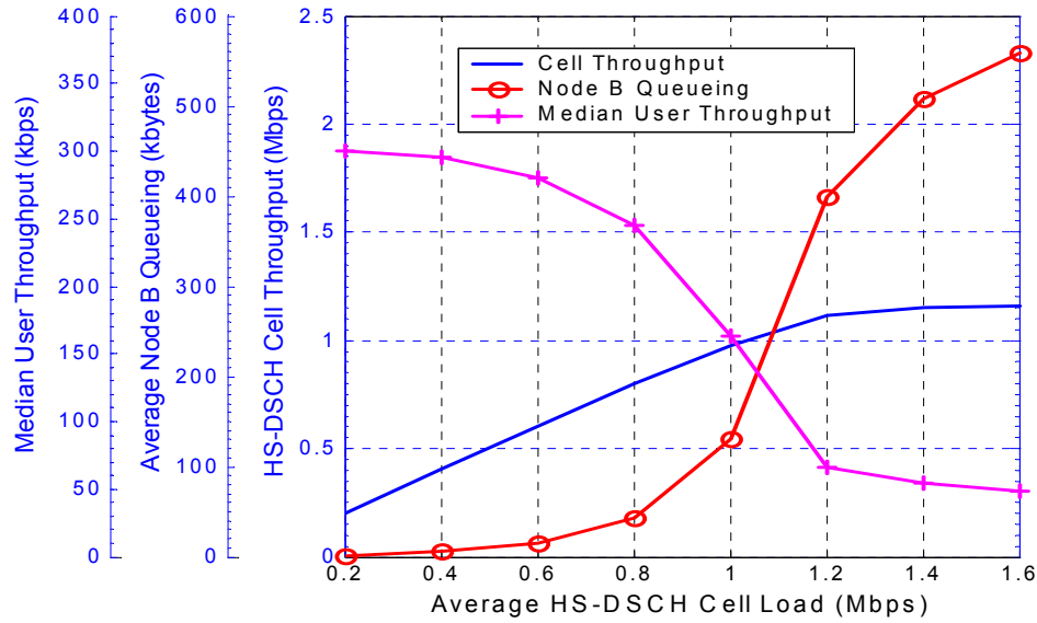
Figure 6.4: Median User Throughput, Average Node B Queueing and HS-DSCH Cell Capacity as a function of the Offered HS-DSCH Cell Load for Round Robin Scheduler in Pedestrian A, 3km/h. HSDPA Power \approx 50% of Total Node B Power & 7 Multi-codes.
