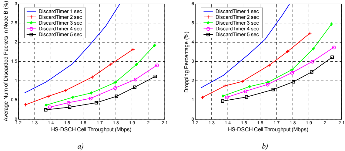
Figure 7.8: a) Percentage of RTP Packets Discarded in the Node B and b) Dropping Rate for 128 kbps CBR Bearers in Ped_A 3km/h, Total Node B Buffering of 20 Mbits, Initial UE Buffering of 5 sec.
