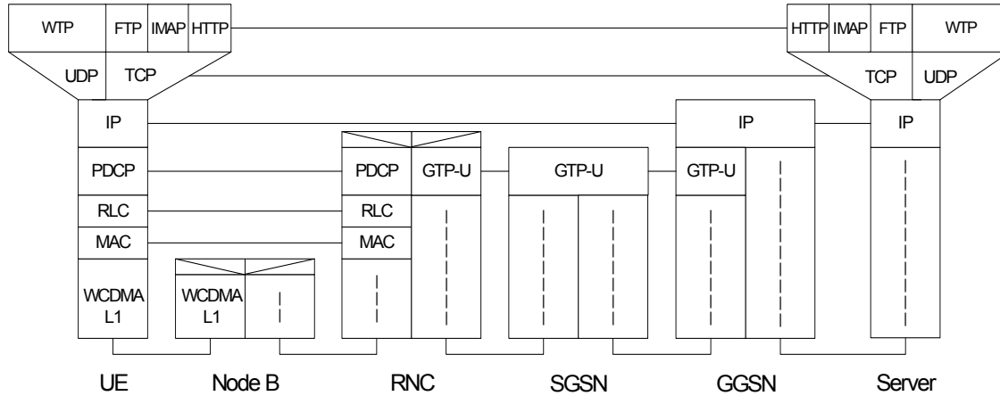
Figure 2.8: Protocol Stack of a NRT Packet Switched Session in UMTS Release 99 Architecture.
