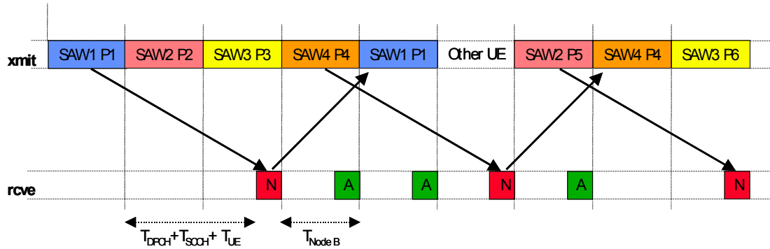
Figure 4.6: Four Channels SAW Protocol Operation. (Timing not in Scale).
