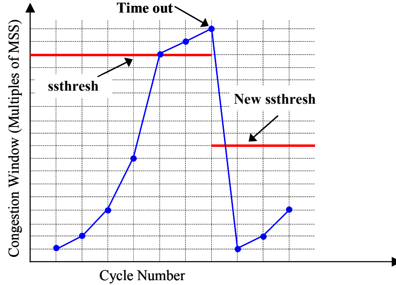
Figure 3.1: Congestion Window Evolution During Slow Start And Congestion Avoidance.
