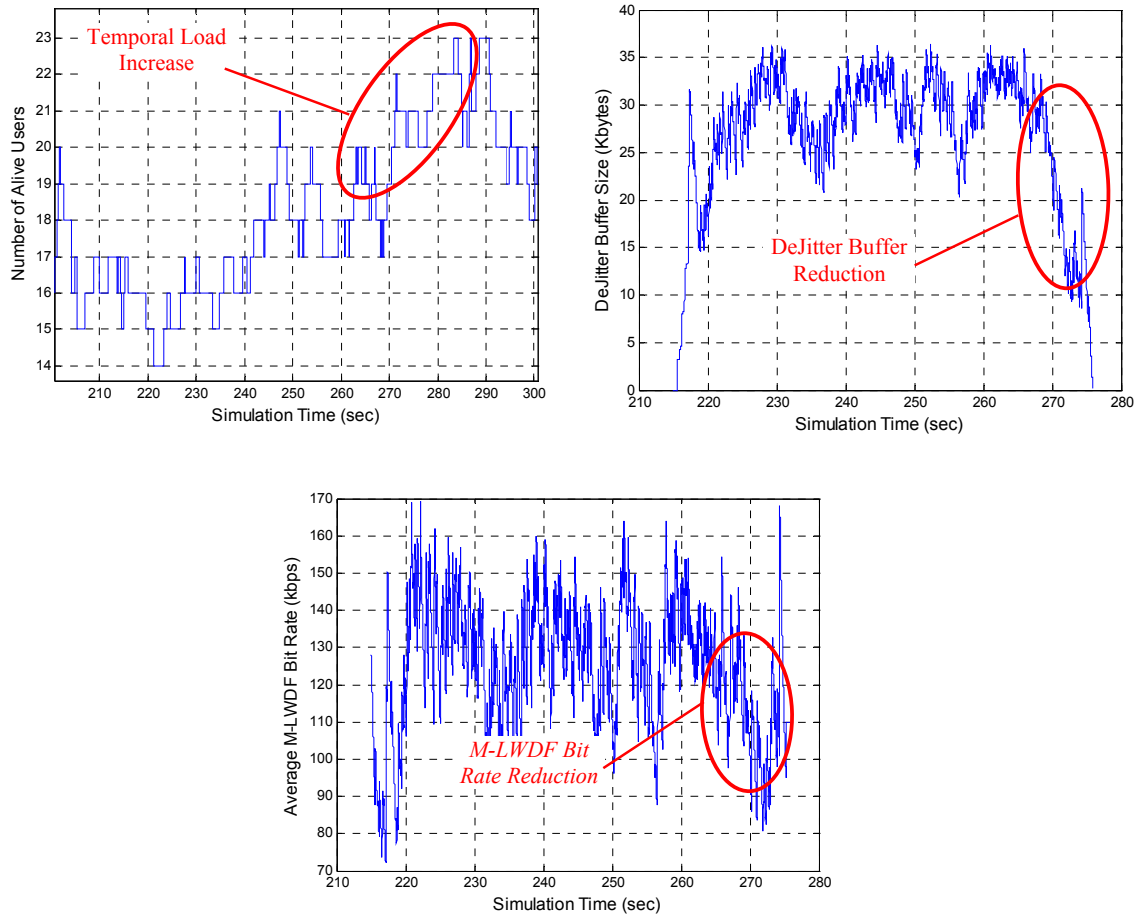
Figure 7.2: Instantaneous Number of Alive Users, DeJitter Buffer Size and Average M-LWDF Bit Rate for a UE with G Factor below -2dB, Average Source Bit Rate 128 kbps, Discard Timer 2 sec, and Initial DeJitter Buffering 1.8 sec.
