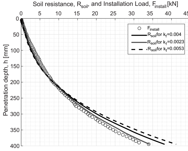
Fig. C.3: Soil resistance compared with installation load
