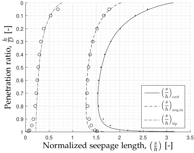
Fig. A.10: Results of \left(\frac{s}{h}\right) for exit, average inside and tip hydraulic gradients for case (c) with \frac{z_L}{D} = 1.0
