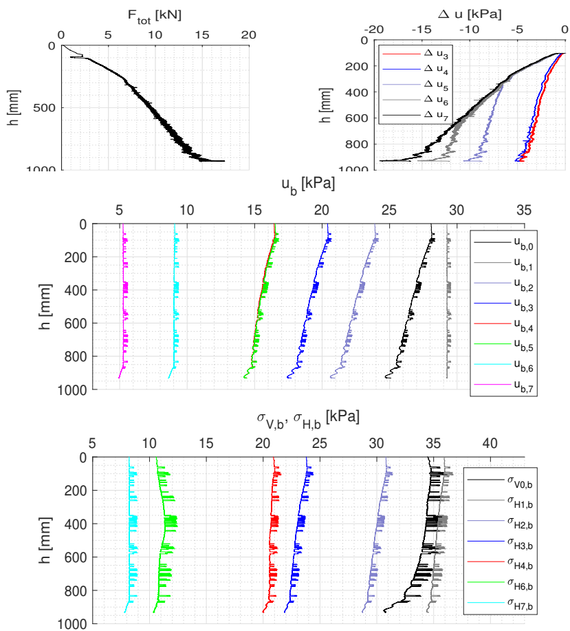
Fig. F.73: Results of installation test
