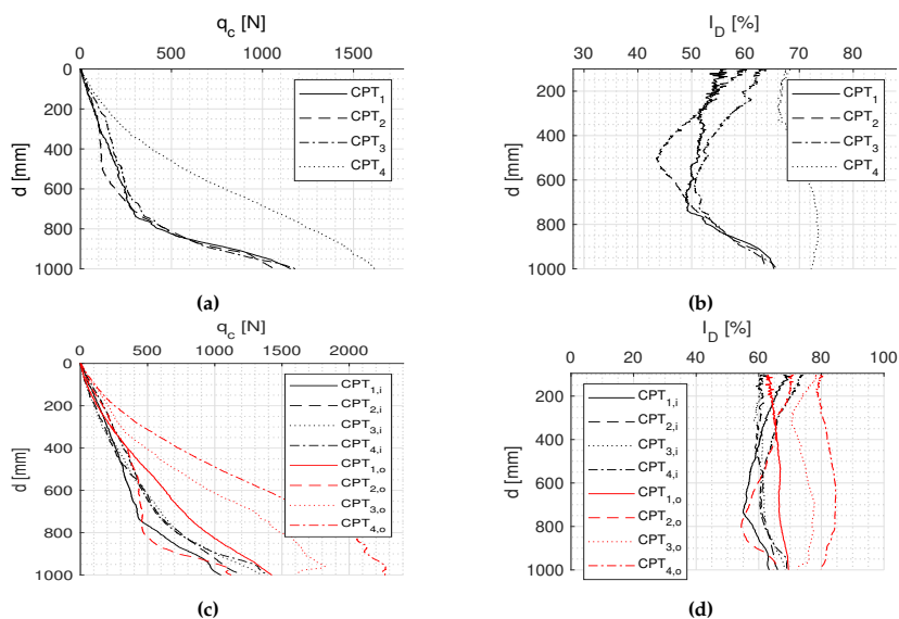
Fig. E.76: Results of CPT (a-b) before installation and (c-d) after installation
