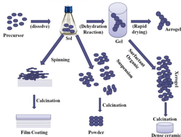
Figure 2-4. Procedures of sol-gel method. Figure reproduced from ref. (35).
