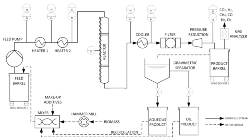
Figure 10. process flow diagram of the CBS1 pilot plant (46).
