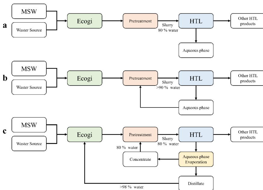
Figure 9. a) Typical HTL process without valorization of the aqueous phase, b) HTL process with direct aqueous phase recirculation, and c) HTL process with recirculation of concentrated aqueous phase.
