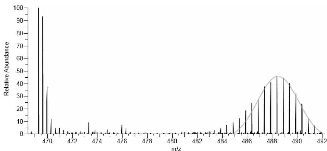
Fig. 3. Example of an MS1 isotope profile for the peptide [NILVNHIVAATLK + 4H]^{4+} of a hypothetical protein from Methanothermobacter with a slightly negative skewness, indicating indirect ^{13}C substrate metabolization (von Bergen et al., 2013). A Gaussian curve has been plotted on top of the isotope profile to highlight the skewness. Example taken from the incubation with ^{13}C -labelled BD at timepoint 120 h.
