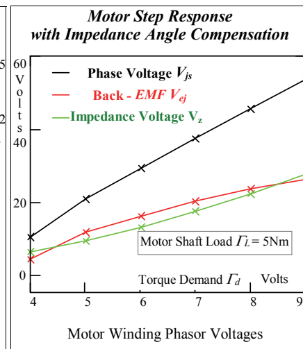
Fig. 28. Phasor Voltages with MIAC
