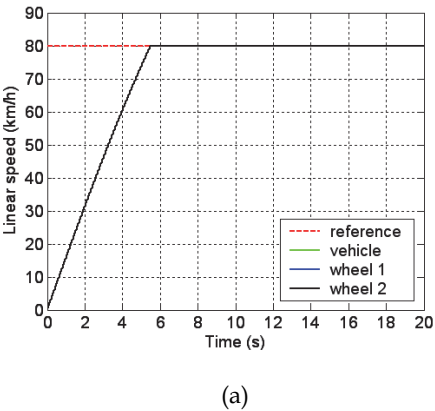
Fig. 25. Simulation results for case 2
