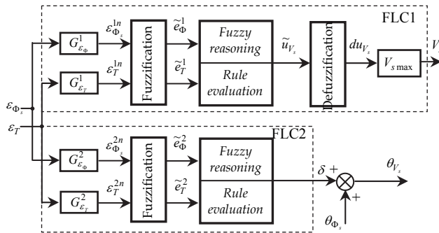
Fig. 11. Fuzzy logic controller structure
