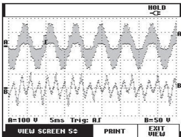
Fig. 13. Measured wave form of armature EMF and axial coil EMF when 2400rpm
