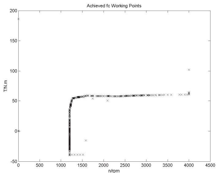
Fig. 3. Working points of ICE
