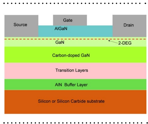
Figure 3-5 | Structural schematic of a basic lateral GaN-HEMT power semiconductor
