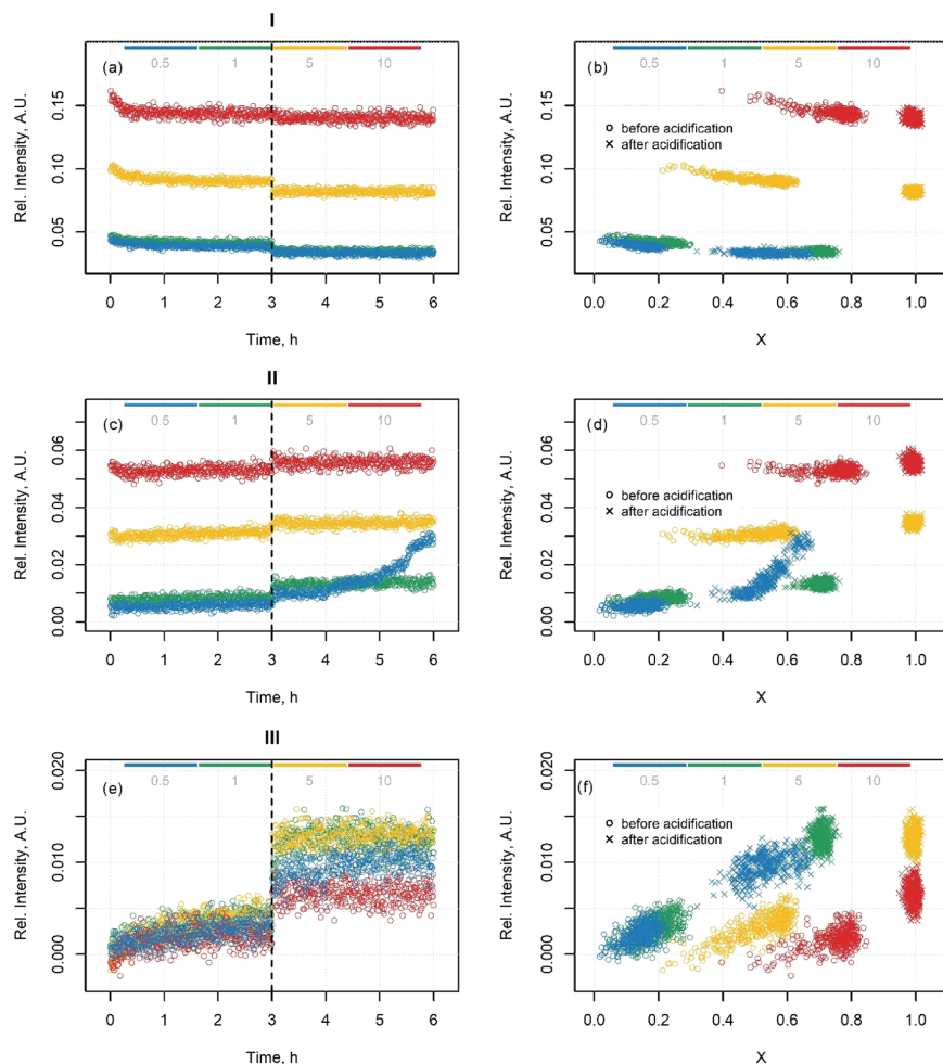
Figure 7. Relative intensity of peaks for executions at \text{pH}_0 = 9 as a function of time (a, c, e) and as a function of \text{HS}^- fractional conversion (b, d, f) for HET (I), DTZ (II), and MEA (III).
