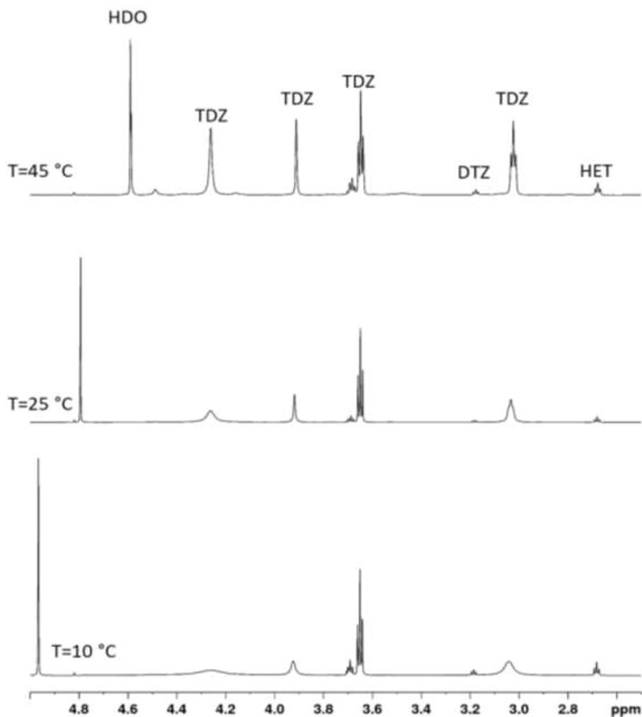
Figure S4. ^1\text{H} -NMR spectra (600 MHz) of TDZ at different temperatures. The resonances of TDZ clearly show a temperature-dependent line broadening which is indicative of chemical exchange at an intermediate timescale comparable to the chemical shift differences between the two forms. All spectra are referenced to internal TSP- \text{d}_4 .
