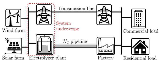
Fig. 1. Electricity-hydrogen combined power system for efficient renewable energy utilization..
