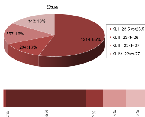
Figur 3.2: Hus 28: Timefordeling i komfortklasser for sommersituation i stue i 2010.
