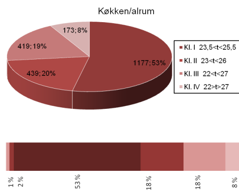
Figur 3.3: Hus 47: Timefordeling i komfortklasser for sommersituation i stue i 2011.
