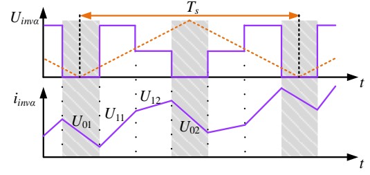
Fig. 21. Diagram of PWM voltage and current.
