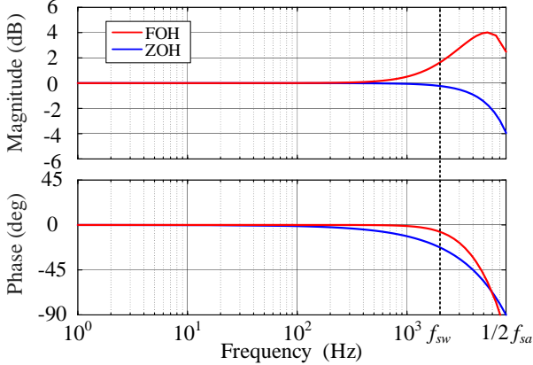
Fig. 13. Bode diagram of the zero-order hold and the first-order hold.
