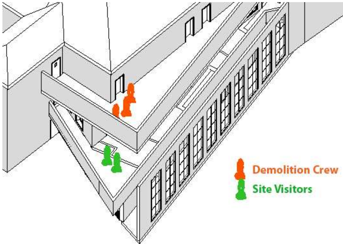
Figure 3. RFID + BIM Virtual Prototype Environment Development Strategy
