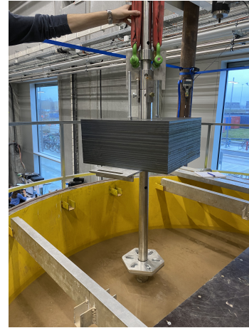
Figure 10. Hammer test configuration
