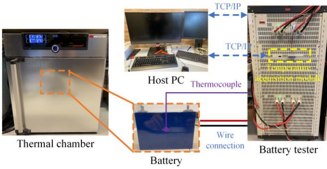
Fig. 3. Experimental setup for parameterization and validation.
