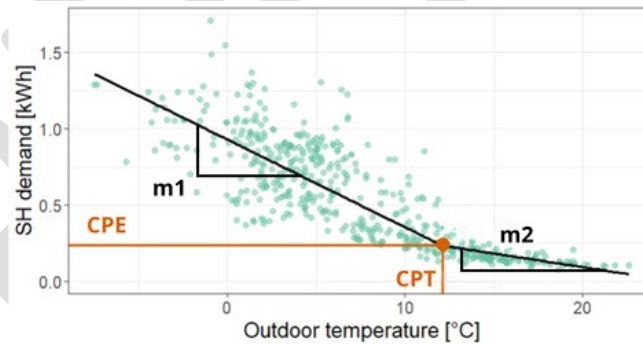
Figure 1: Representation of the ES model for heating purposes.
