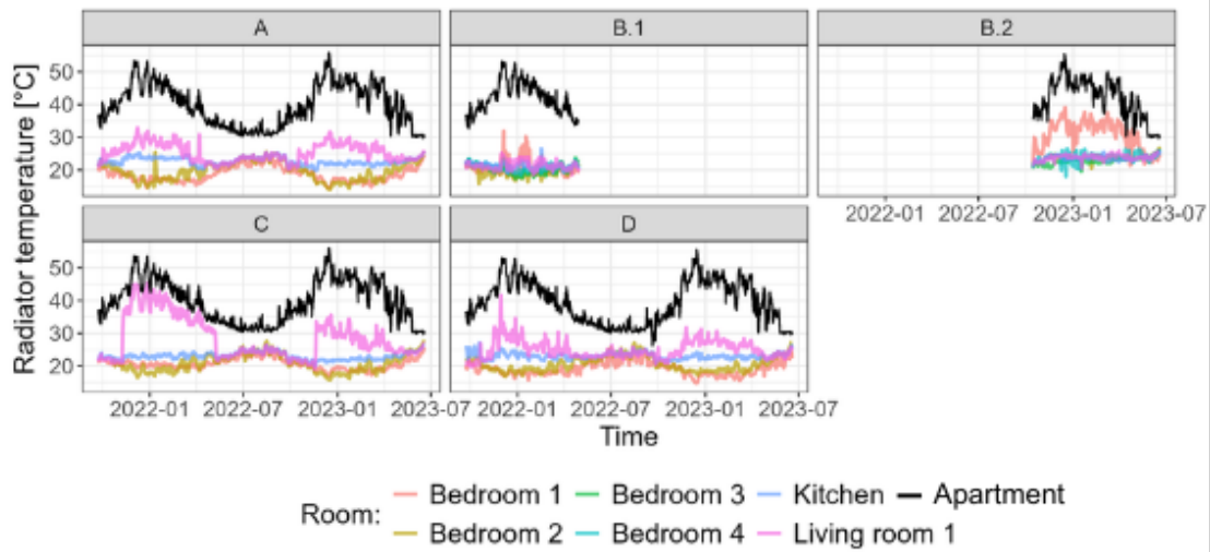
Figure 10: Radiators' temperature per room (colored) compared with the apartment SH supply temperature (black).
