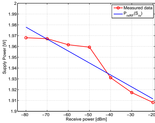
Fig. 4. Receive RF.
