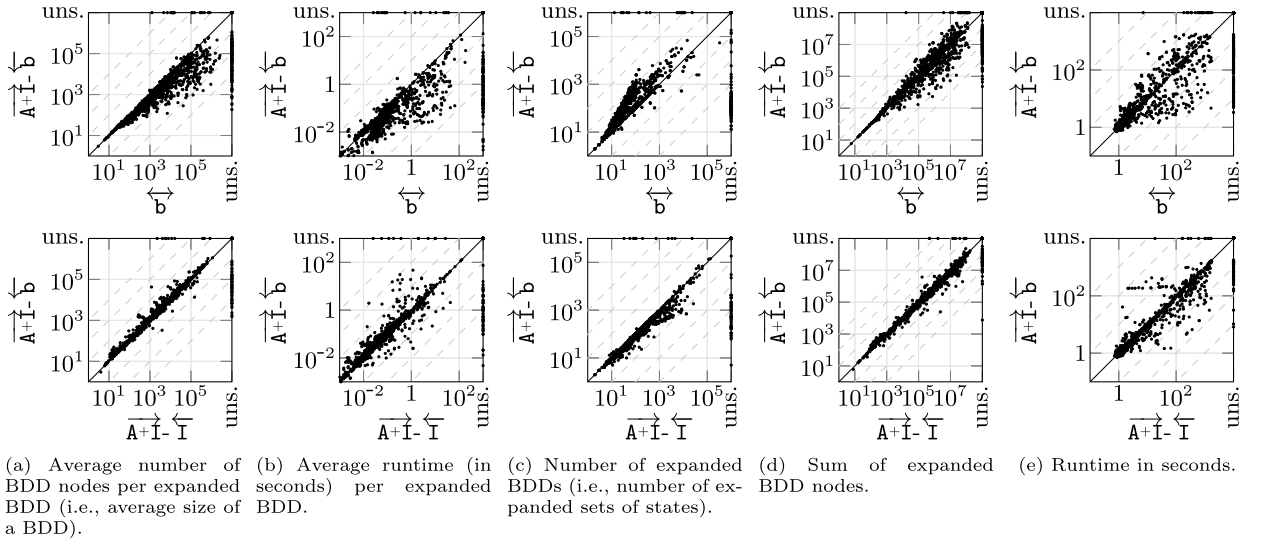
Fig. 10. Per-task comparison between the best-performing variant of backward GHSETA* ( \overline{I} ) and the backward blind symbolic search ( \overline{b} ).
