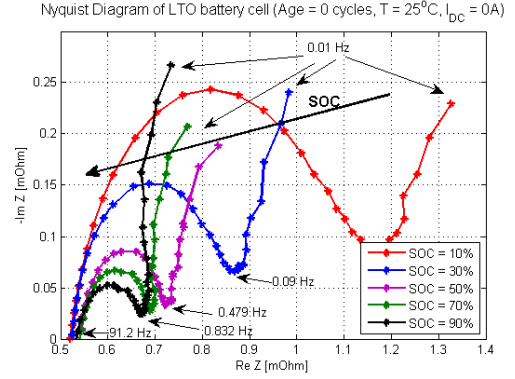
Fig. 2. Measured impedance spectra of the LTO battery cell for different SOC's at 25^\circ\text{C} .
