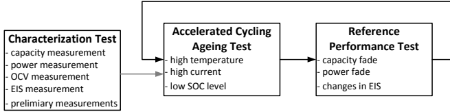
Fig. 1. Accelerated ageing procedure for the LTO battery cell.
