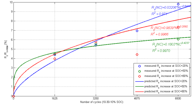
Fig. 13. Effect of the age on the value of R_s for different SOC.
