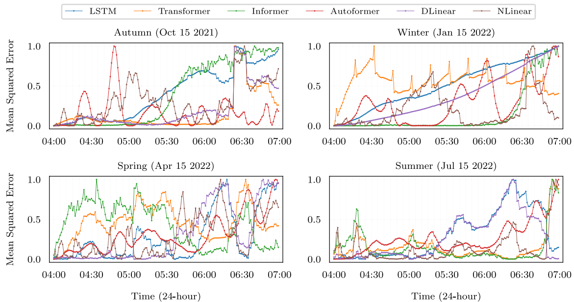
Fig. 11. Step-wise mean squared error of all models for the four data points in different sequences.
