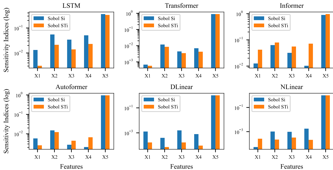
Fig. 9. Sobol sensitivity indices (logarithmic) of the P amount in the prediction to each one of the input features for all models, where X1, X2, X3, X4, and X5, represent the metal dosage, NH_4 , NO_3 , NH_4 + NO_3 , and PO_4 , respectively.
