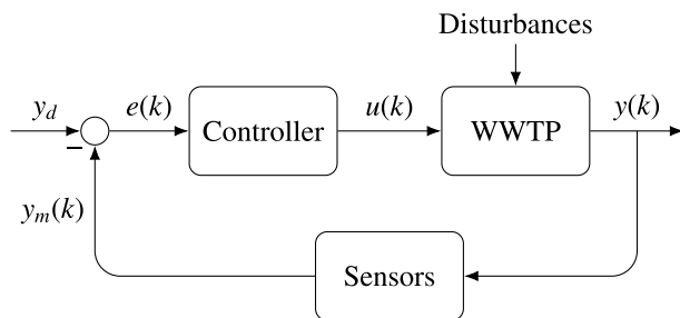
Fig. 2. The control block diagram of the system.
