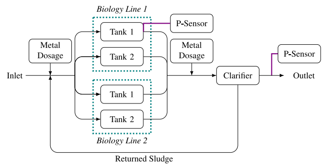
Fig. 1. Schematic of the phosphorus removal process in the plant with the flow lines: The iron salt is added to the inflow to the biological tanks, where P is removed, and a sensor in Tank 1 measures phosphate. There is a dosage of polyaluminium chloride before the secondary settler to remove the remaining P, and the final phosphate concentration is measured at the outlet.
