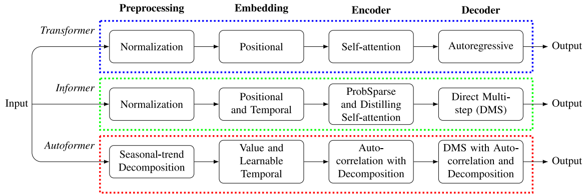
Fig. 4. The structures of encoder–decoder attention-based models ( Transformer (Vaswani et al., 2017), Informer (Zhou et al., 2021)), and auto-correlation ( Autoformer (Wu et al., 2021)) for time series forecasting tasks.
