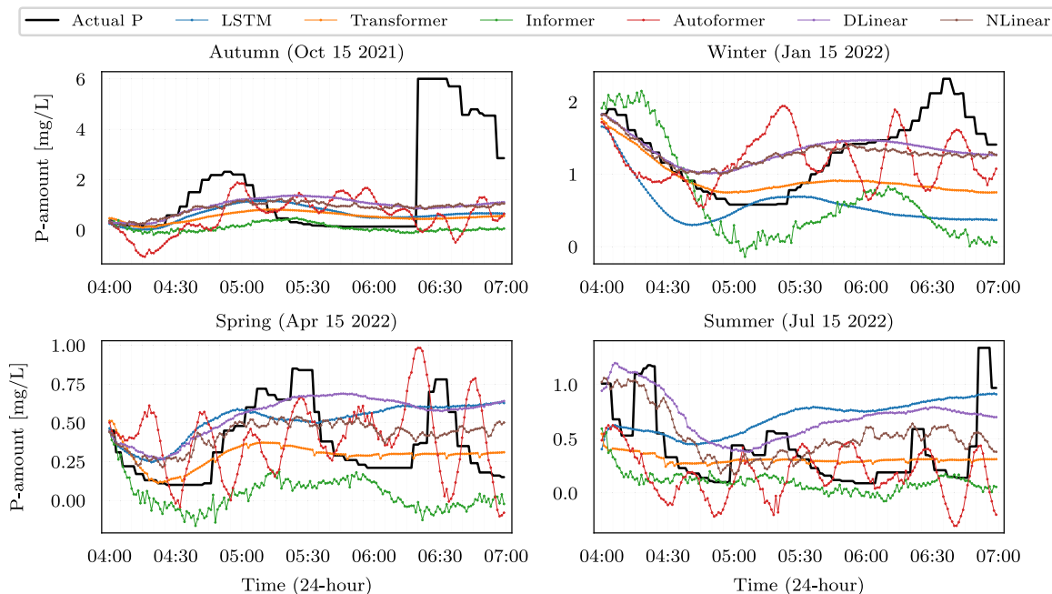
Fig. 10. Simulation environment results of all models for the four data points in different sequences.
