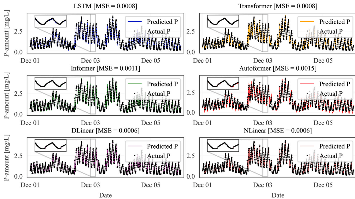
Fig. 8. Prediction results of all models for a part (5 days) of the test dataset.
