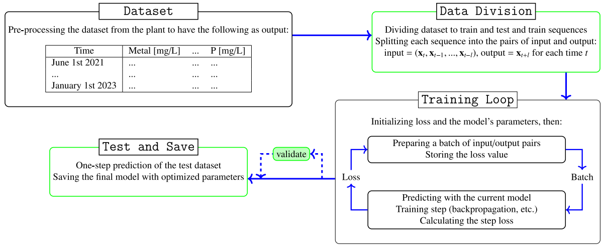
Fig. 6. The procedure of training, testing, and saving a model for the prediction of future time steps of the plant's data.
