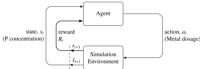
Fig. 7. The process of a testing simulation environment for one model in a specific time point.
