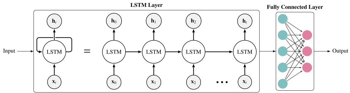
Fig. 3. The structure of the LSTM (Hochreiter and Schmidhuber, 1997) model for time series forecasting tasks, where (x_0, \dots, x_r) , and (h_0, \dots, h_r) represent the input and the hidden state (output) of each LSTM cell.
