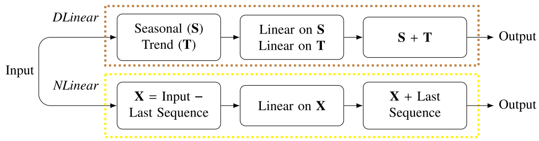
Fig. 5. The pipeline of LTSF Linear (Zeng et al., 2022) models ( DLinear and NLinear ) to forecast time series.
