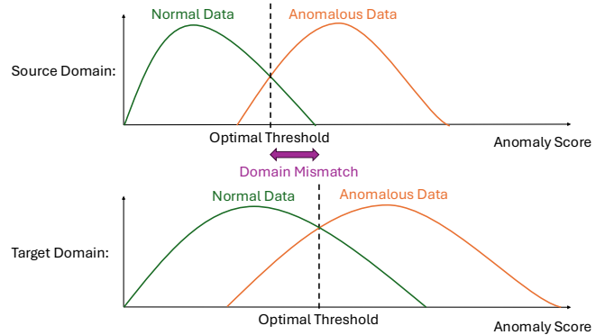
Fig. 1. Illustration of the domain mismatch between the anomaly scores of a source domain and a target domain.
