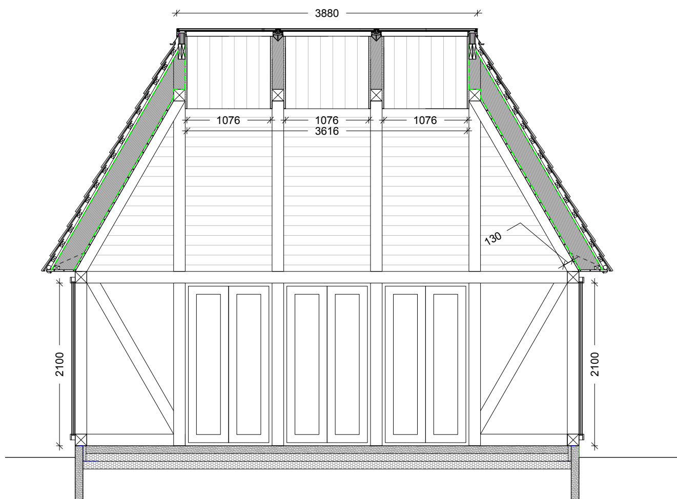
LANG SNIT 1:50
