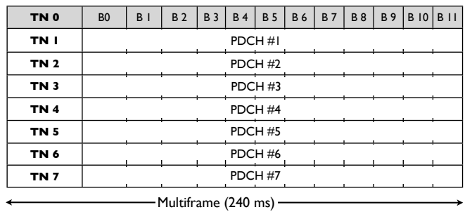
Fig. 2: Multiframe structure composed by 7 time slots (TN0 to TN7) and 7 Packet Data Channels (PDCH).
