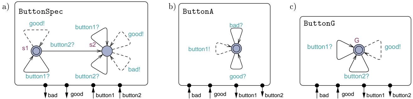
Figure 9: Specification of a) the ButtonSpec , b) the assumption ButtonA , c) the guarantee ButtonG .
